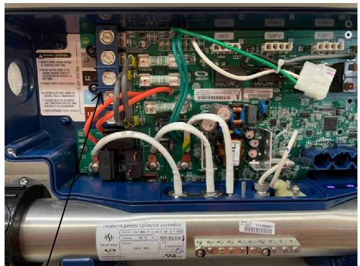
Terminal Block
